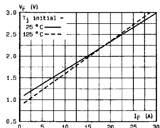
Figure 6. Voltage drop versus forward current.
