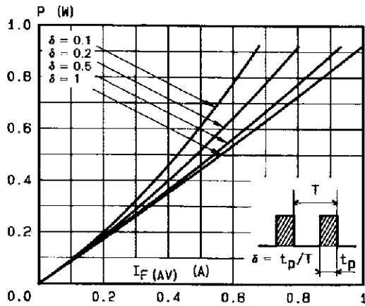
Figure 1. Power losses versus average current.
